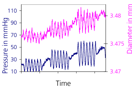
Applied pressure and strain response of a vessel
